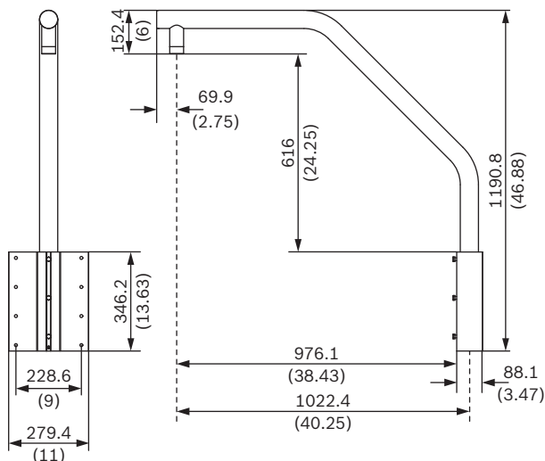
VGA-ROOF-MOUNT 尺寸
