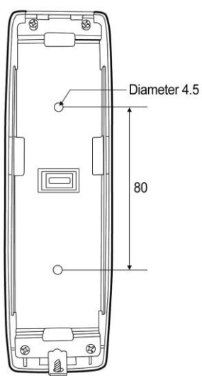
Extension Bracket
