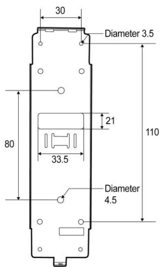
Basic Bracket
