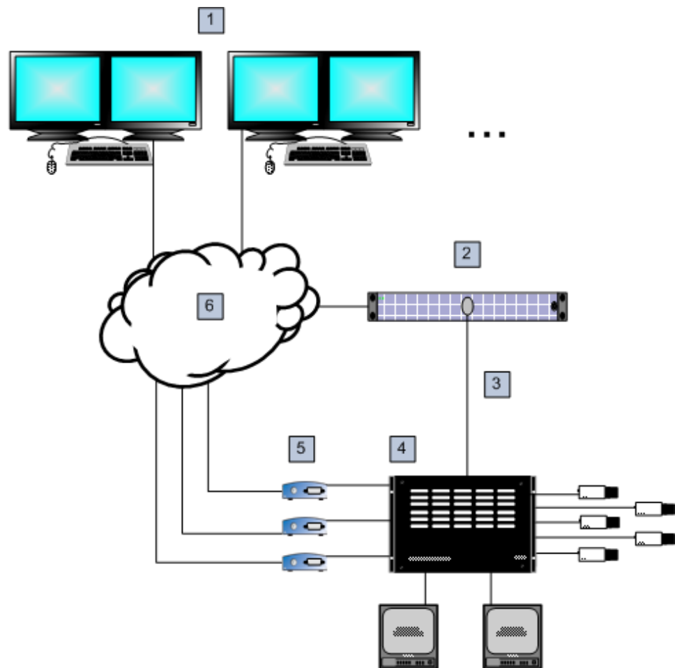
Figure 5.6: Connexion locale de Bosch Video Management System à la matrice Allegiant Bosch
