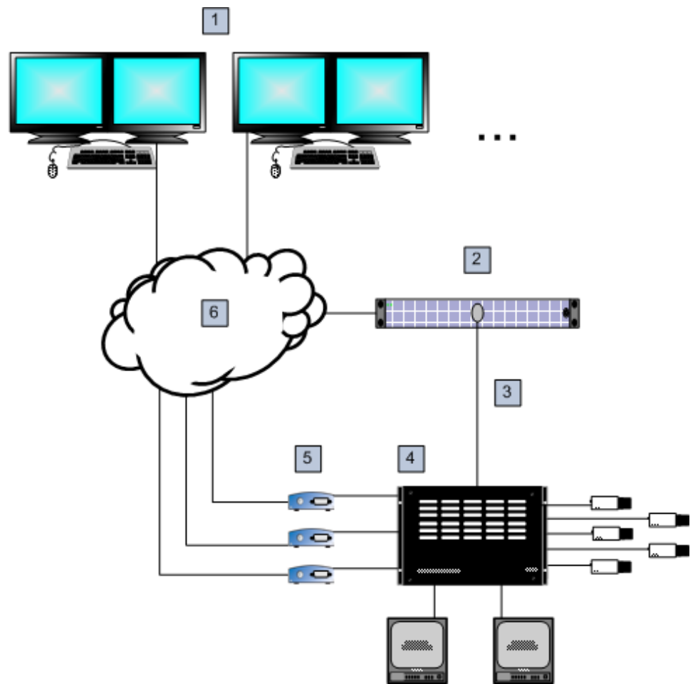
图 5.6: Bosch Video Management System 与 Bosch Allegiant 矩阵切换台的本地连接
