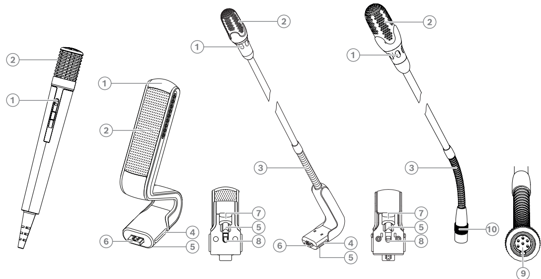
Abbildung 7.26: DCNM-FHH / DCNM-FHHC, DCNM-HDMIC, DCNM-MICS / DCNM-MICL und DCNM-MICSLL / DCNM-MICSLs
