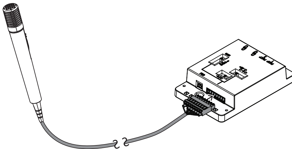
Figura 7.17: Collegare DCNM-FAI a DCNM-FHH/DCNM-FHHC
