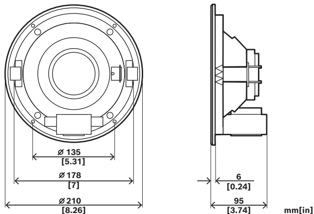
Abb. 1: Abmessungen (in mm)
