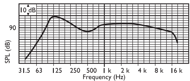
Abb. 4: Frequenzgang
