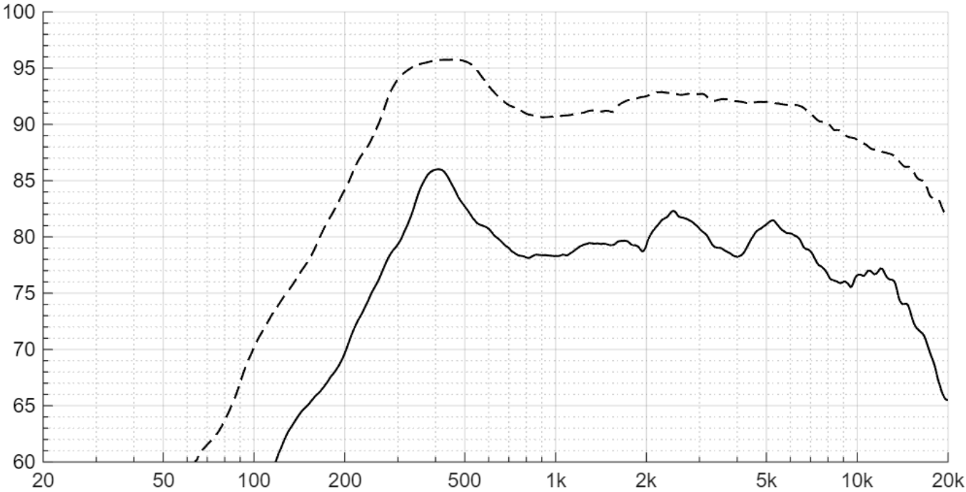
Fig. 2: Frequency response graph — 1/3rd octave dB SPL @1 W(20 Hz — 20 kHz), 4 m -- 1/1th octave dB SPL @1 W(20 Hz — 20 kHz), 1 m.
