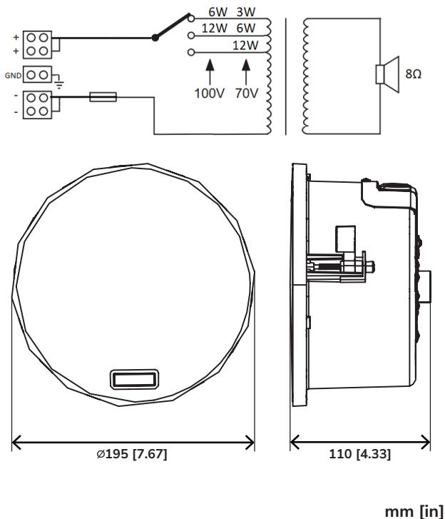
Fig. 1: Dimension
