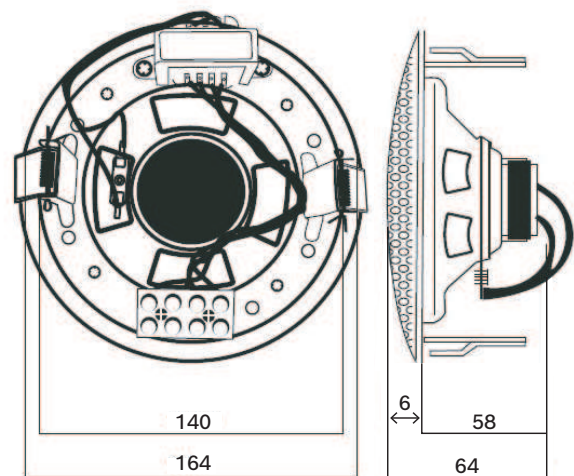
Fig. 1: Dimensions in mm
