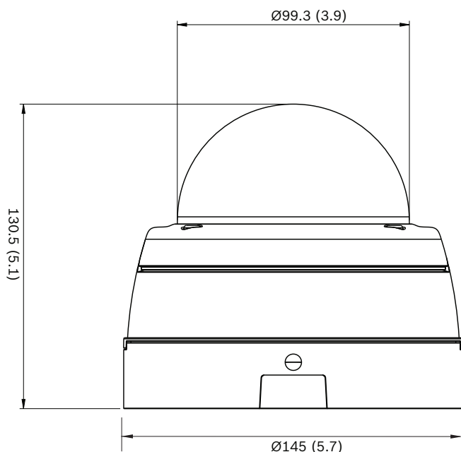
Fig. 1: Dimensions (mm)
